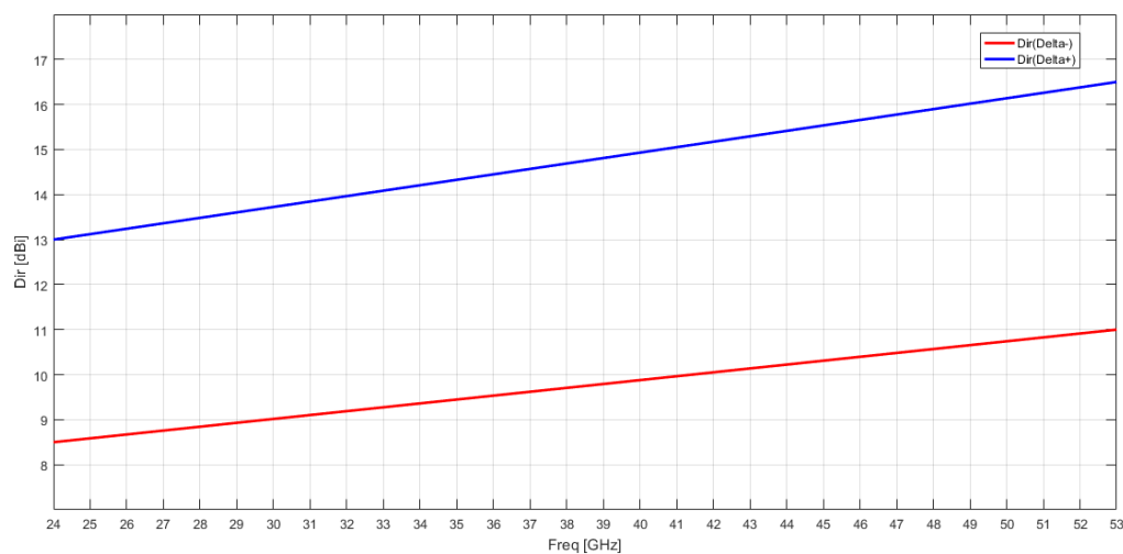
Figure 7.2-1 Directivity Mask
