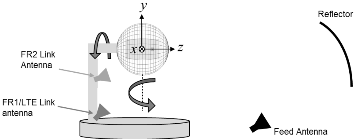
Figure 2.1.2-1 Example of IFF: CATR Measurement Setup
