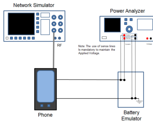
Figure 4.1-1 Energy Use Per Activity Test Setup
