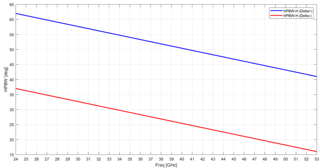
Figure 7.2-3 HPBW-H Mask
