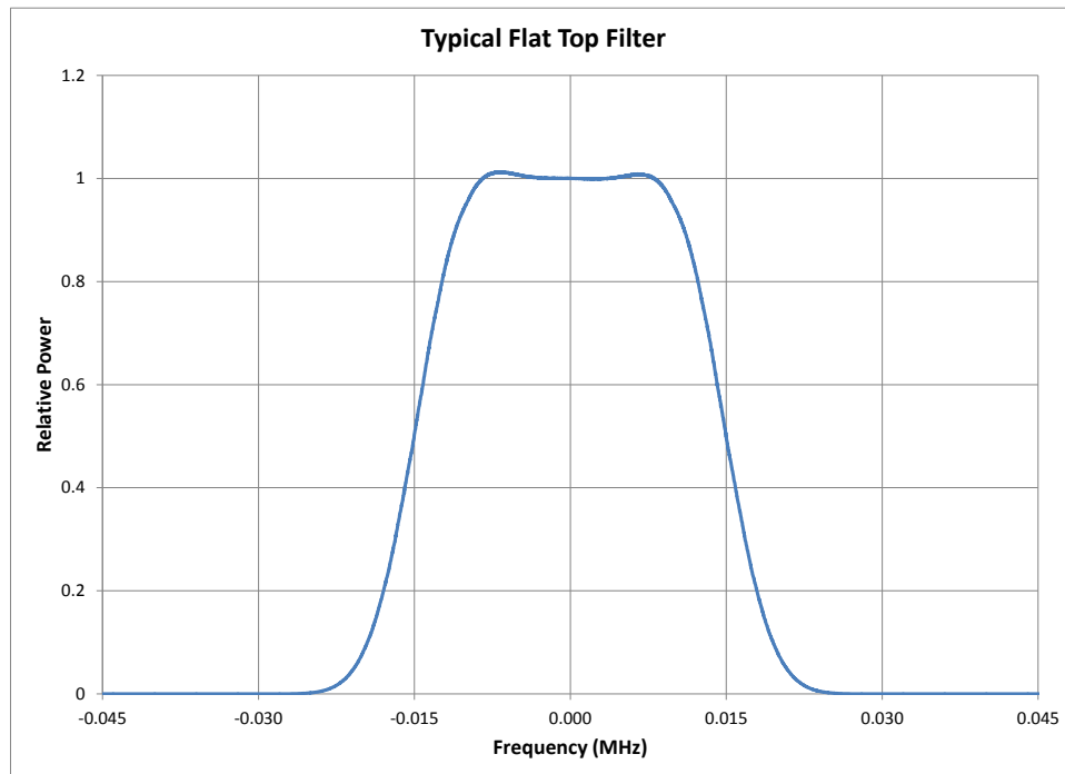
Figure 9.5.1-3 Example of a Flat Top Filter with 30 KHz RBW
