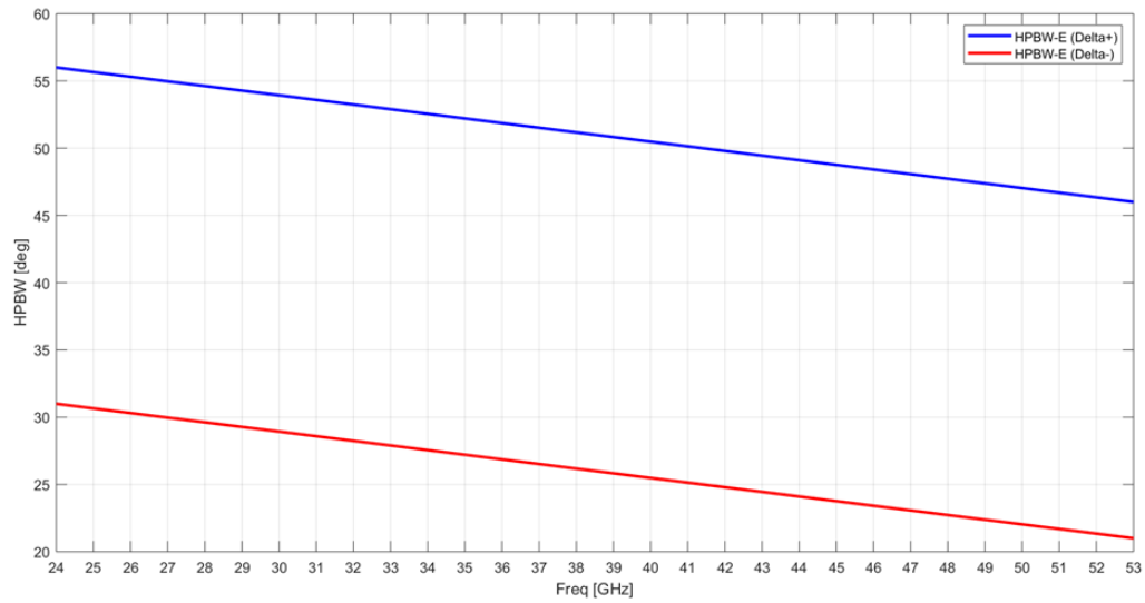
Figure 7.2-2 HPBW-E Mask
