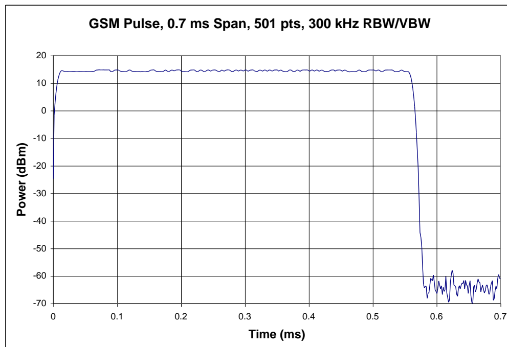
Figure 9.7-1 Sample GSM Power Envelope with Acceptable Resolution
