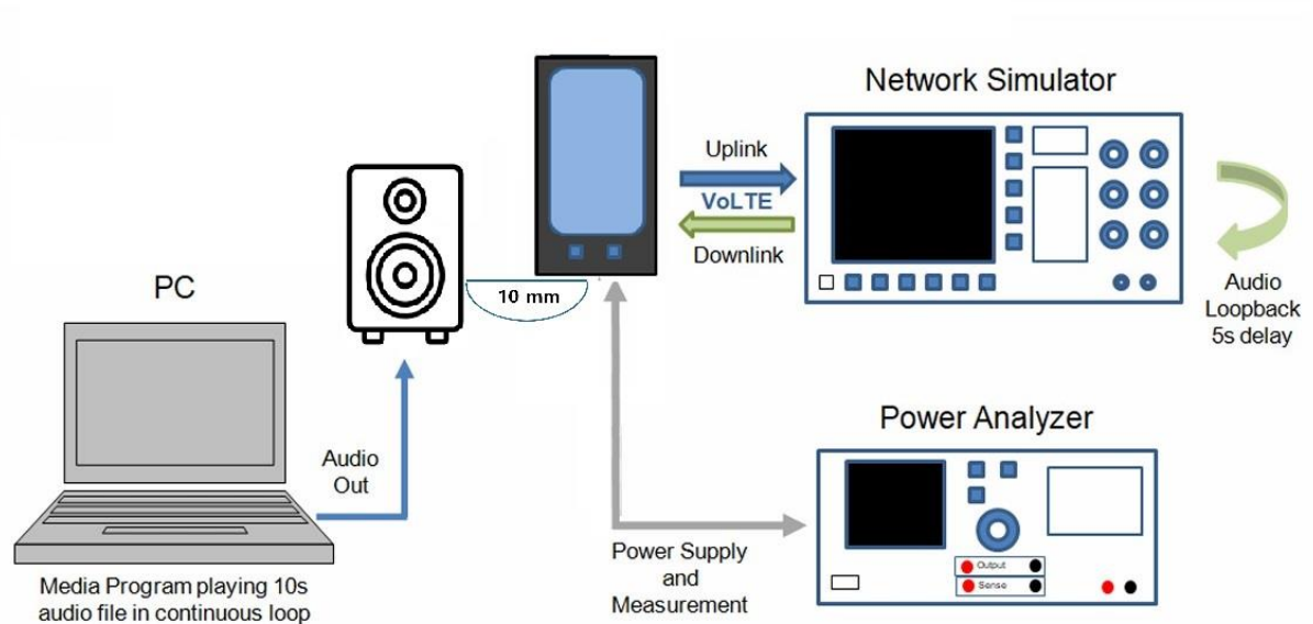
Figure 4.2-1 VoLTE/VoNR Test Setup
