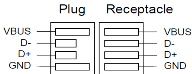
Figure 3 Charging Downstream – Detection Signaling
