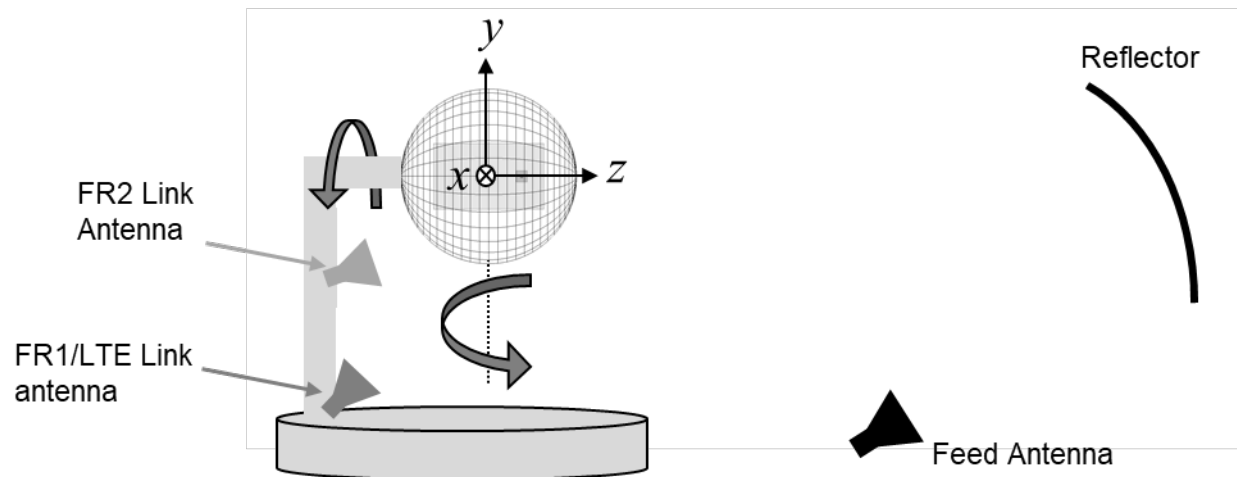
Figure 2.4-3 Example of IFF: CATR Measurement Setup
