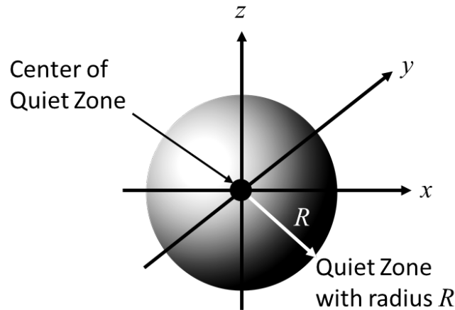
Figure 3.4-1 Quiet Zone Illustration
