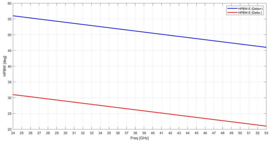
Figure 3.2-3 HPBW-H mask
