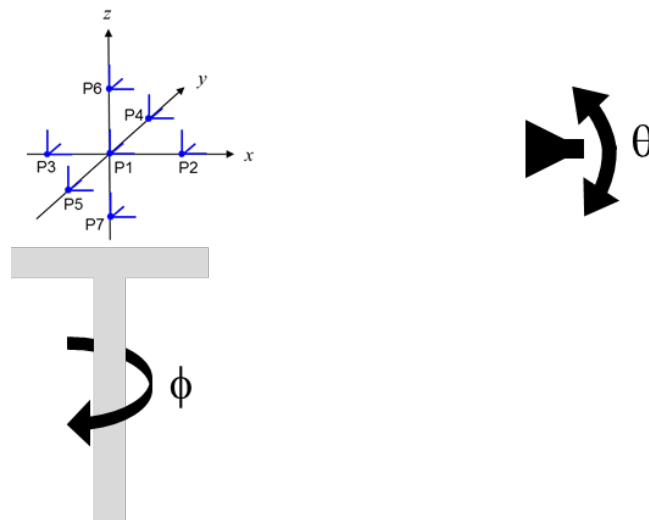
Figure 3.5-3 Reference AUT Measurement Positions for Distributed-Axes System
