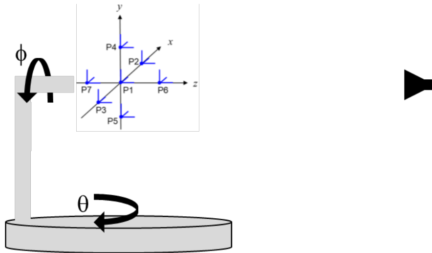
Figure 3.5-5 Reference AUT Measurement Positions for combined-axes System
