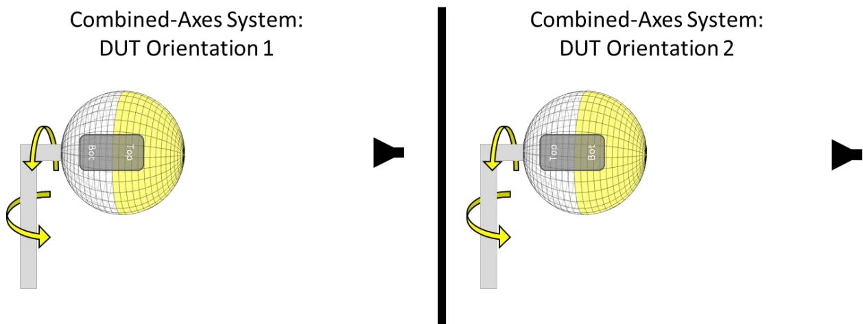
Figure 7.7-3 DUT Re-Positioning for an Example of Combined-Axes System
