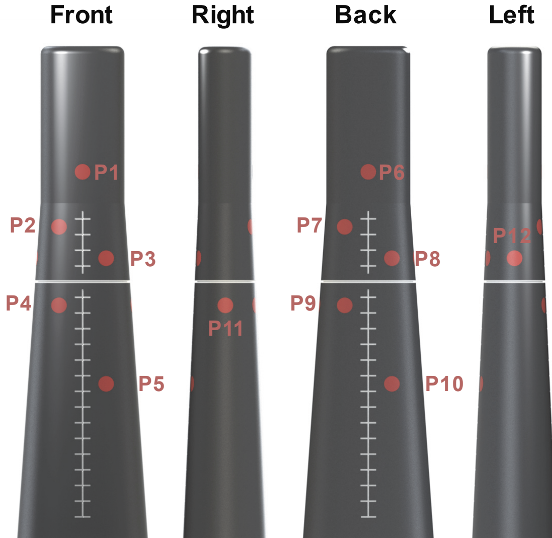
FIGURE G-8 TWELVE LOCATIONS FOR DIELECTRIC MEASUREMENTS ON THE FOREARM PHANTOM
