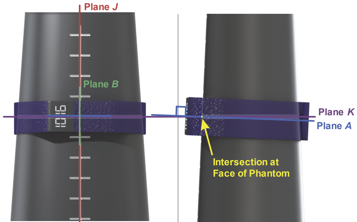
FIGURE Q-7 ALIGNMENT OF PLANE A WITH PLANE K AND PLANE B WITH PLANE J WHEN A WRIST-WORN DEVICE WITH A PRE-FORMED WRIST BAND IS MOUNTED ON THE FOREARM PHANTOM
