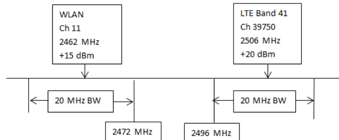
Figure E.1-2 LTE Band 41 and Wi-Fi 2.4 GHz Frequency Diagram
