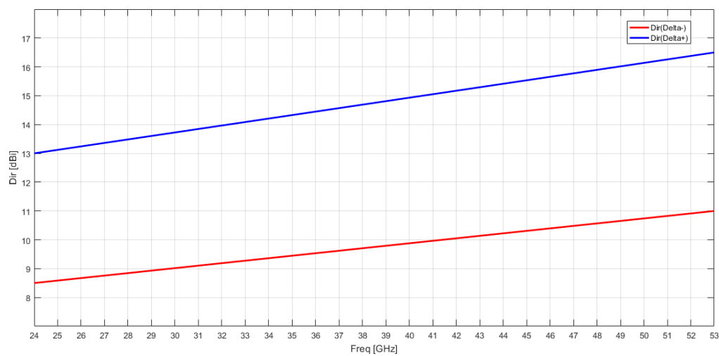
Figure 7.2-1 Directivity Mask
