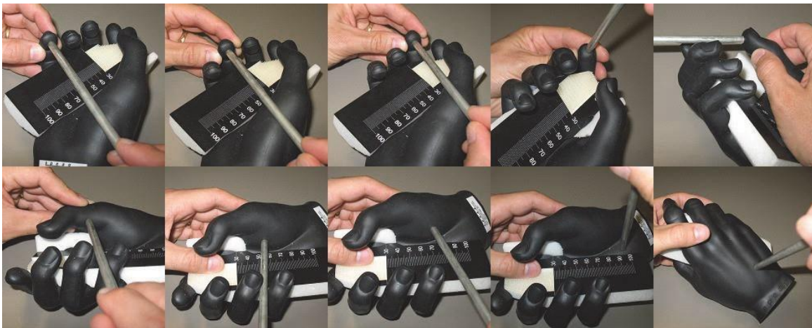
Figure 2.13.2.2-3 Ten Locations of Dielectric Measurements at the Narrow Data Hand Surface
