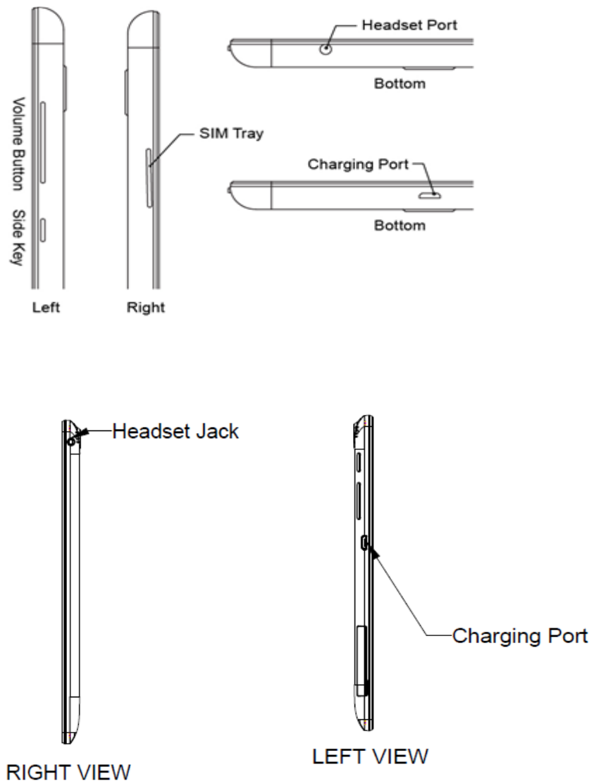
Figure 2.3-10 Side View of Tablets
